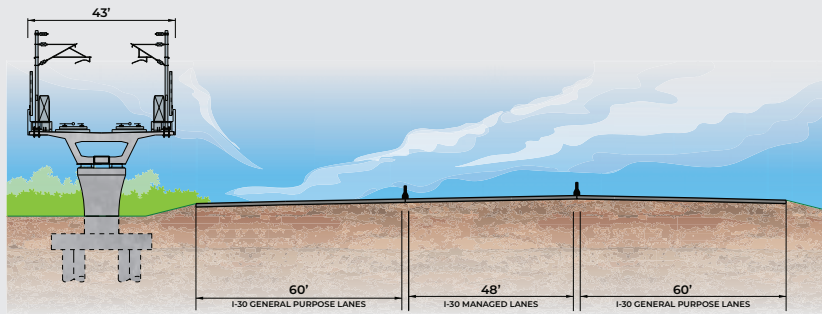
High-Speed Rail I-30 Elevated Typical Section MacArthur Blvd. to Cockrell Hill Rd.
