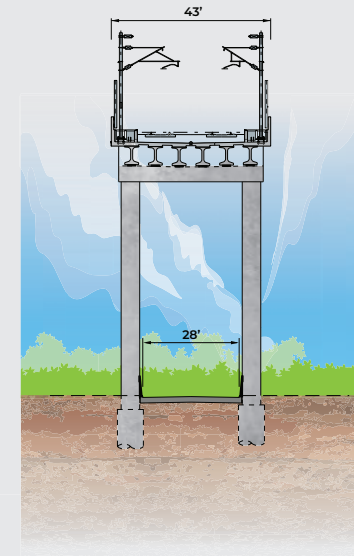
High-Speed Rail Downtown Dallas Two-Column Alternative Typical Section Along Hyatt Regency Hotel Dr. and Hotel St.
