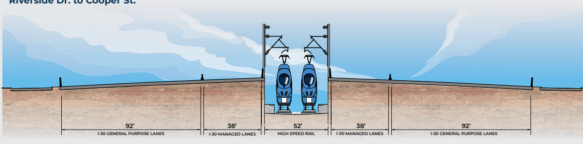
High-Speed Rail I-30 Trenched Typical Section Riverside Dr. to Cooper St.
