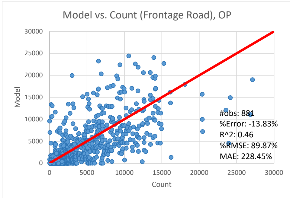
Exhibit 4-33. Scatter plot for frontage road, OP
