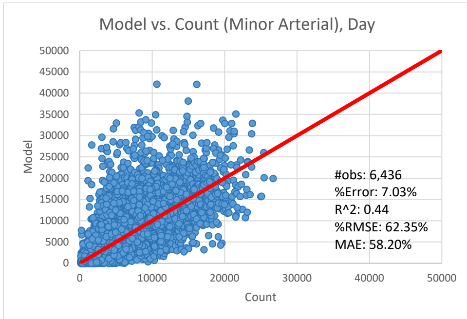
Exhibit 4-18. Scatter plot for minor arterial, day
