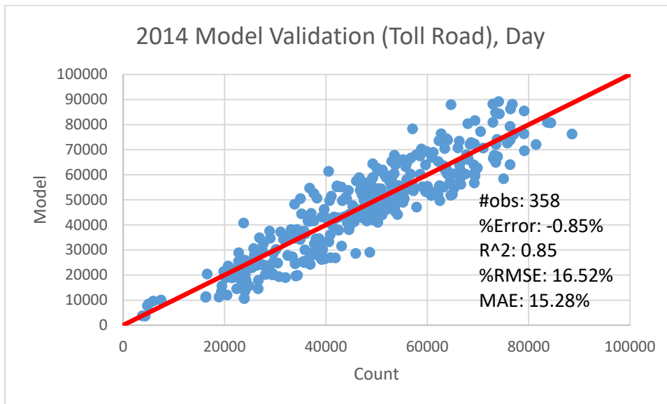
Exhibit 4-39. Scatter plot for toll road, day
