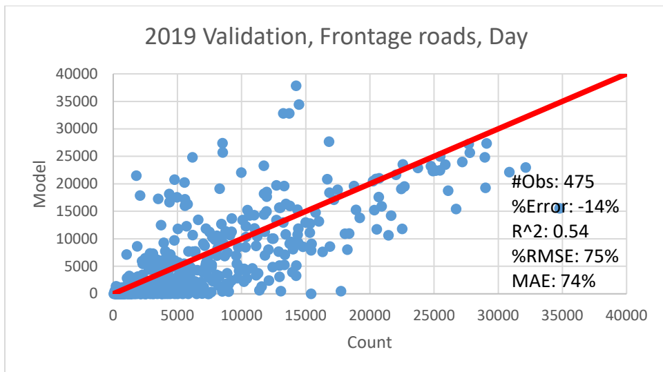
Exhibit 7-9. Scatter plot for frontage roads, day, TAFT model vs. count, 2019 validation
