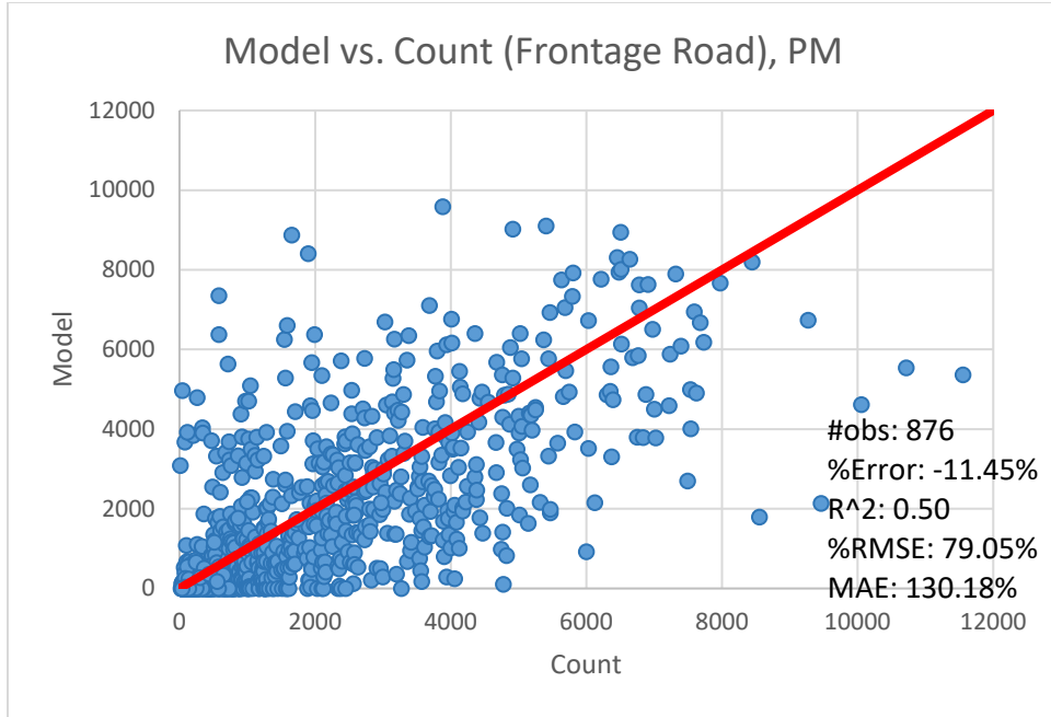
Exhibit 4-32. Scatter plot for frontage road, PM
