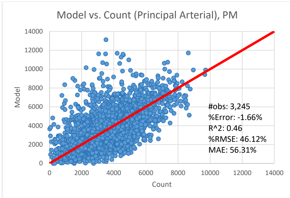
Exhibit 4-16. Scatter plot for principal arterial, PM
