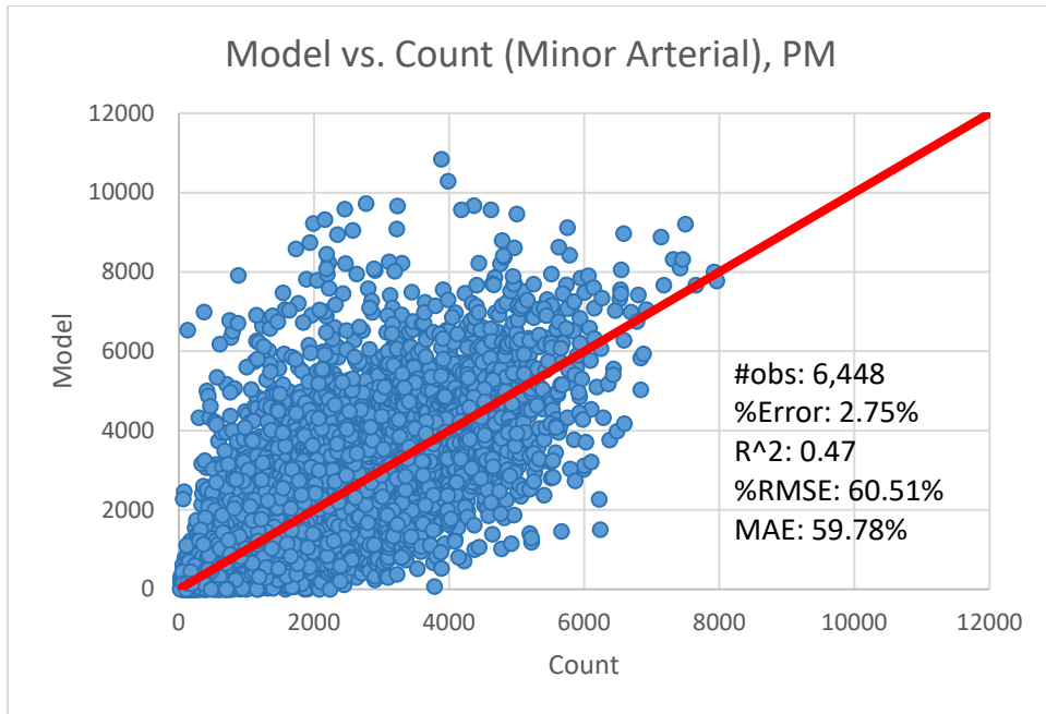
Exhibit 4-20. Scatter plot for minor arterial, PM
