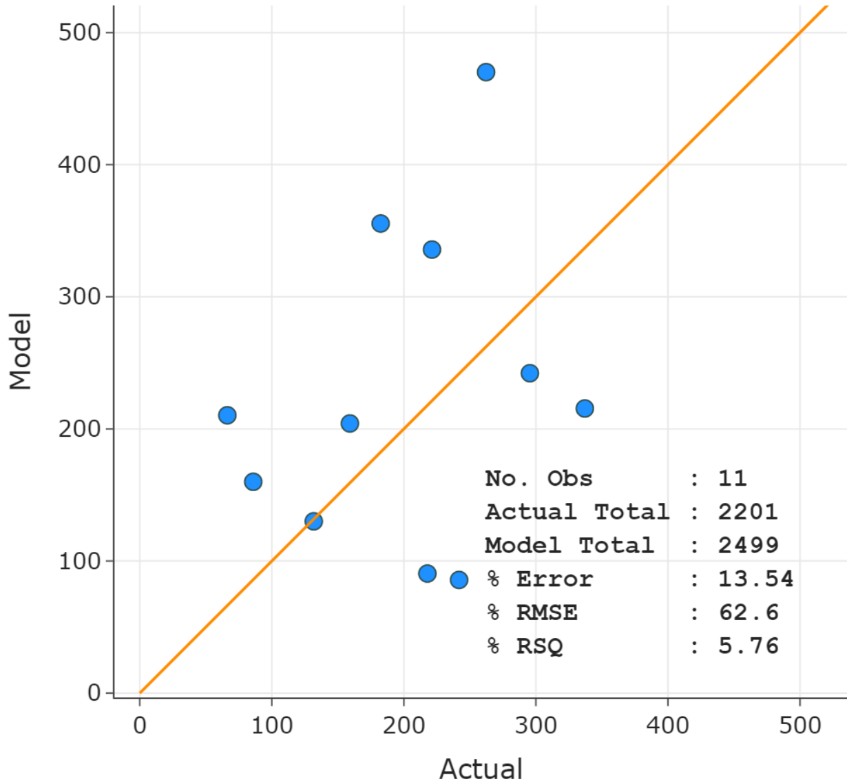
Exhibit Appendix B-5. 2019 DCTA Bus Ridership Comparison – Model vs Actual
