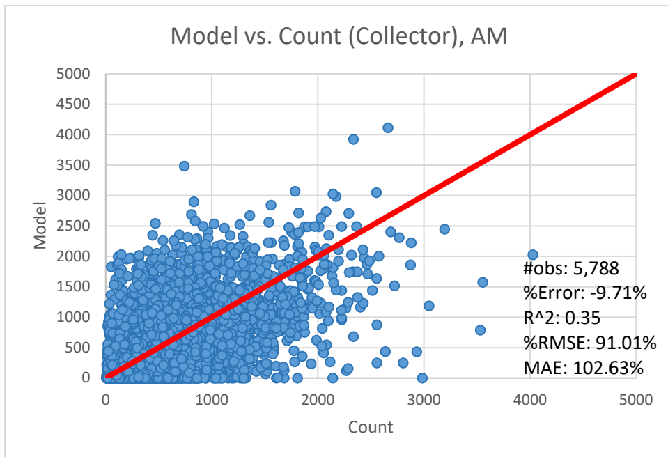
Exhibit 4-23. Scatter plot for collector, AM
