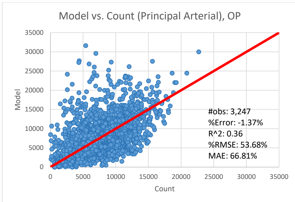
Exhibit 4-17. Scatter plot for principal arterial, OP
