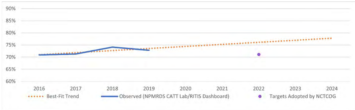
Exhibit IX-13: Latest Observations and Targets for Interstate and Non-Interstate Reliability
