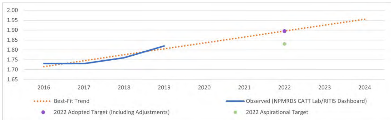
Exhibit IX-16: Observed Data, Trends, and Targets for Truck Travel Time Reliability
